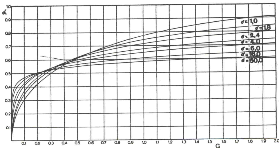
Fig. 7. Influence of particle size distribution on a particular reaction (D1) 8 .
